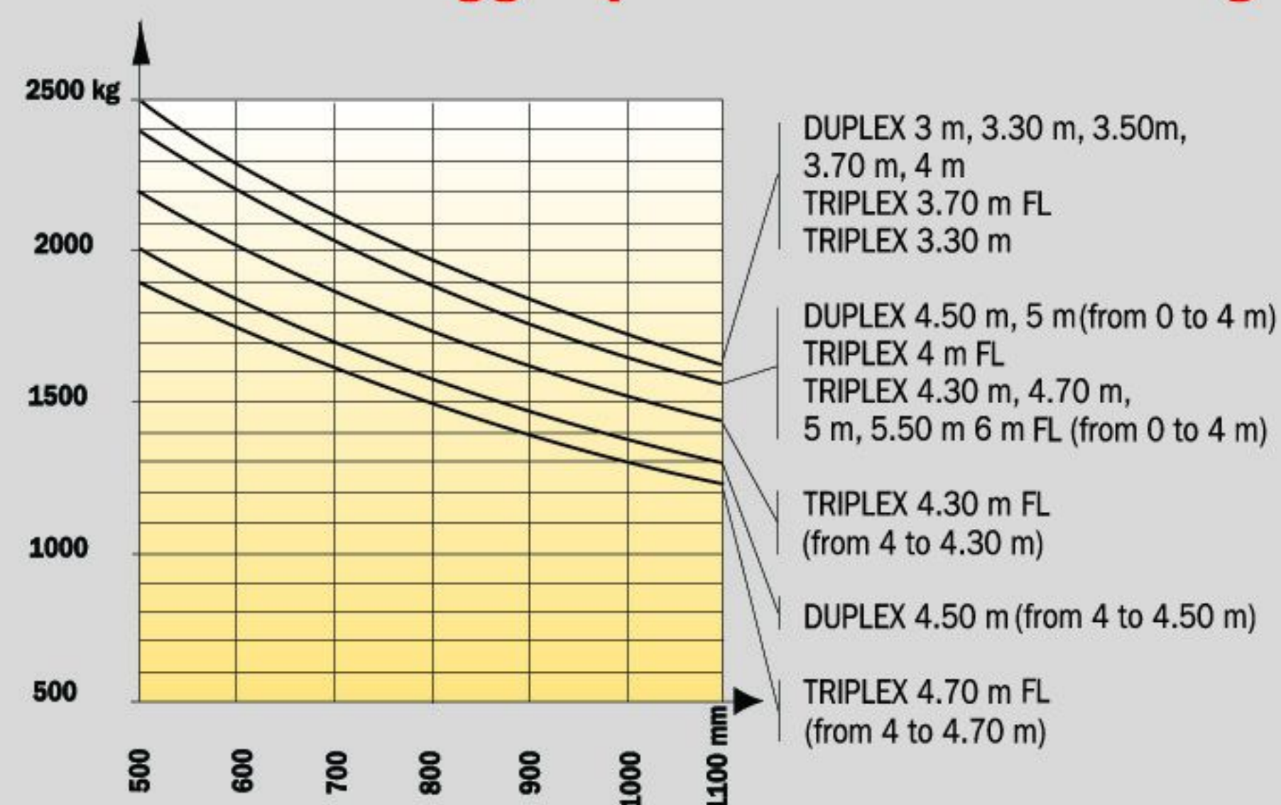
MH 25 - 4 T Buggie (with Side shift carriage)
